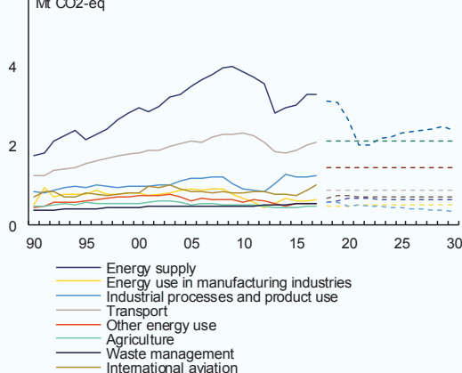
Graph 1b: GHG emissions by sector
