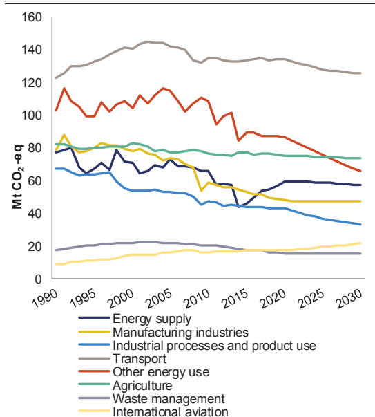
Graph 4.5.2: Greenhouse gas emissions by sector with projections
