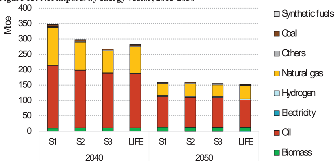
Figure 15: Net imports by energy vector, 2015-2050
