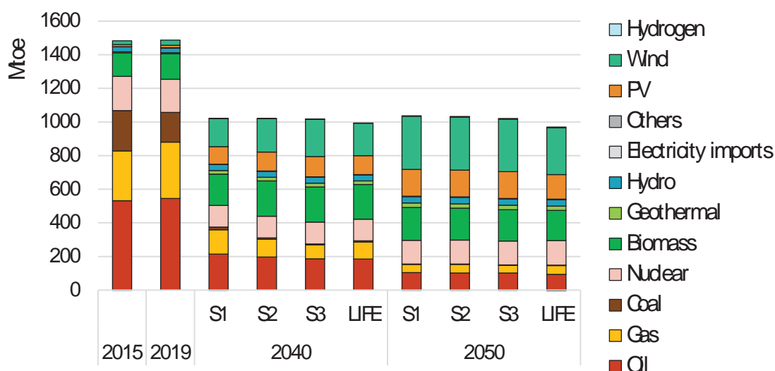
Figure 14: Gross Available Energy by energy vector, 2015-2050
