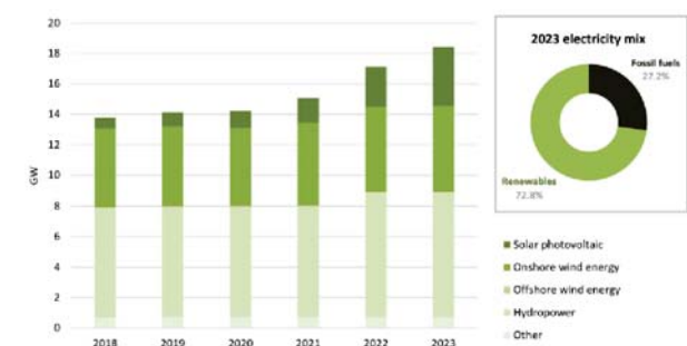
Graph A7.3: Portugal's installed renewable capacity (left) and electricity generation mix (right)
