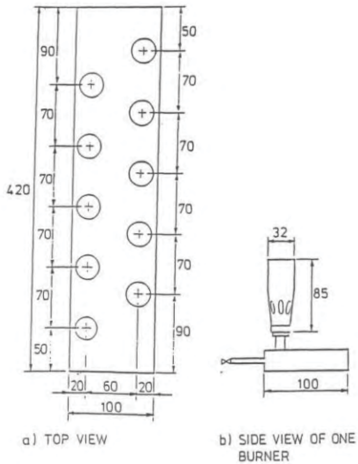
FIG. 1 FIRE ENDURANCE TEST BURNER ASSEMBLY
