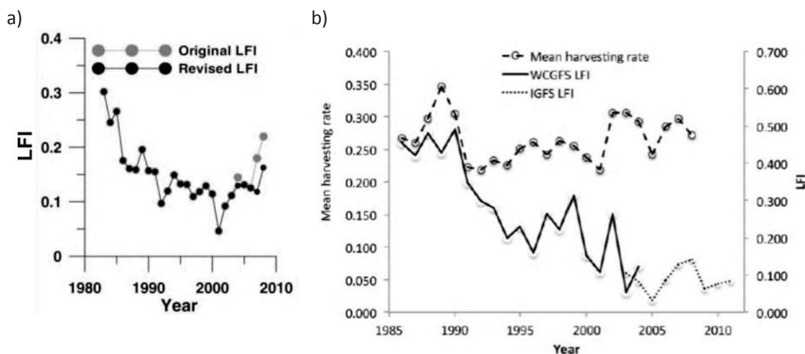
Figure 24: a) LFI trends in the North Sea (Greenstreet et al., 2011) b) in the Celtic Sea. For 1b two overlapping LFI series are shown: the UK West Coast Groundfish Survey (WCGFS) that concluded in 2004, and the ongoing Irish Groundfish Survey (IGFS) (Shephard et al., 2013).
