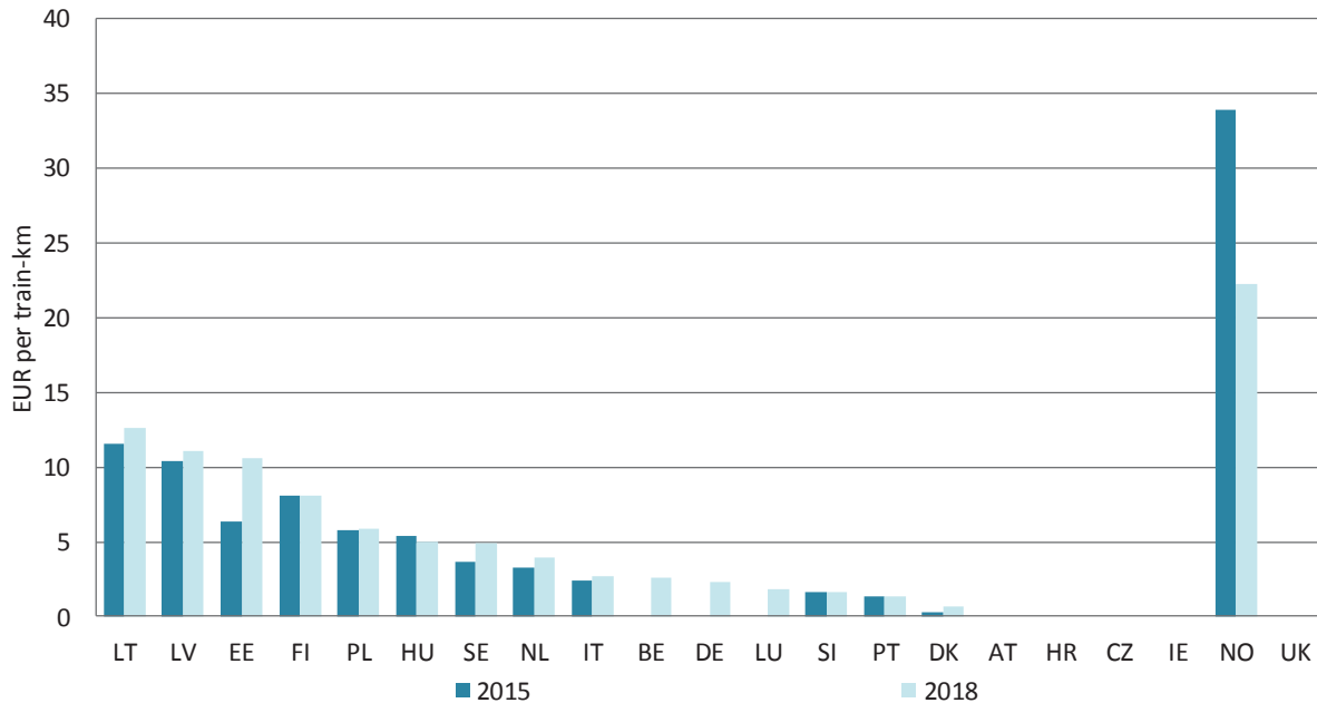
Figure 64: Access charges (excluding mark-ups) for 6 000 tonne freight trains by country (EUR per train-km, 2015 and 2018)
