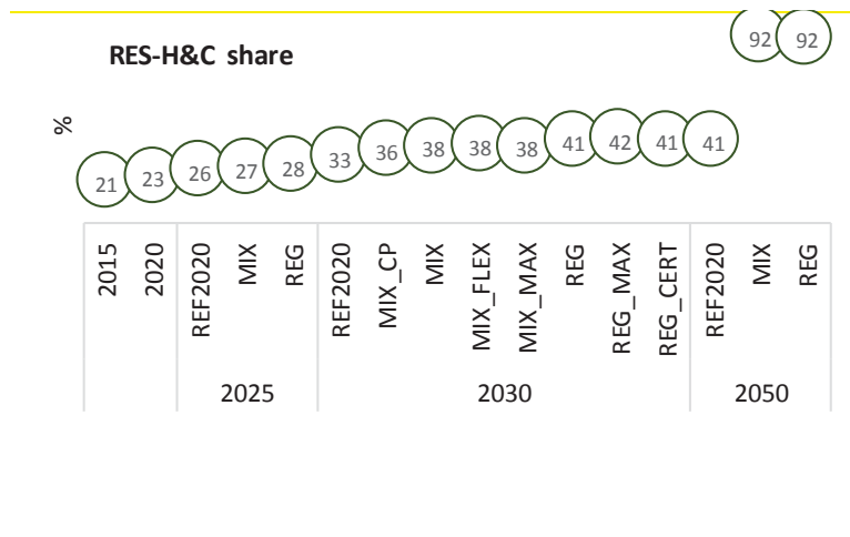
Figure 15: Projection of RES H&C shares.
