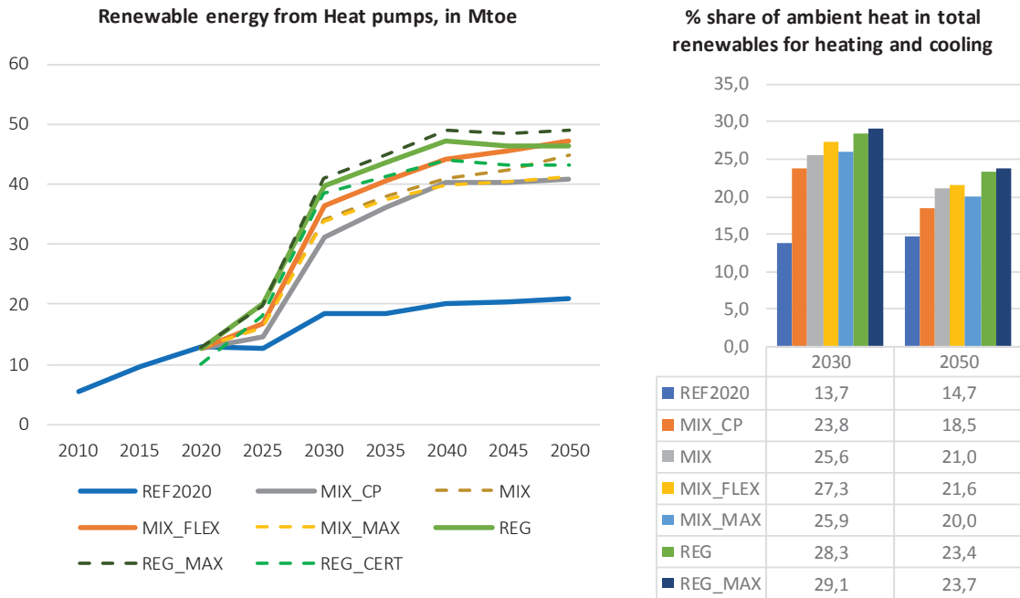
Figure 16: Outlook of ambient heat used in heat pumps.
