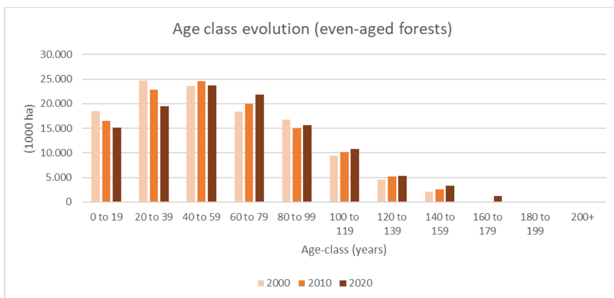
Figure 23 Age class evolution in even-aged forests. Source: Based on Pilli et al., 2016
