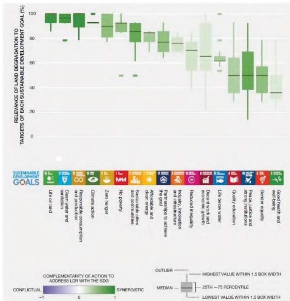
Relevance of land degradation to targets of each SDG Figure 8: addressing soil and land degradation is relevant and synergistic in achieving all the SDGs 154 .
