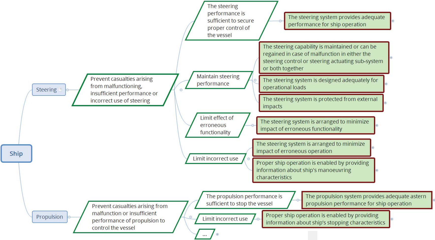
Figure 1 Structure of goals and functional requirements
