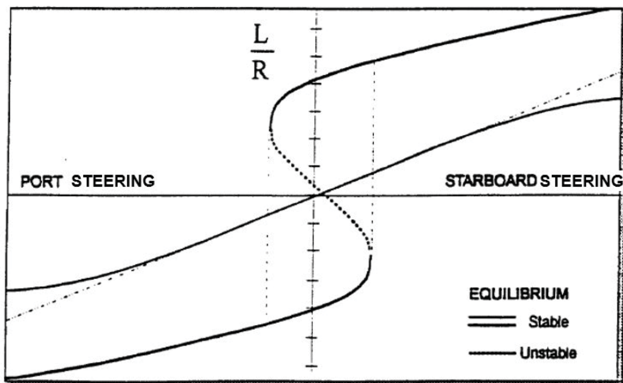
Figure 1 - The equilibrium yaw rate / rudder steering angle relation
