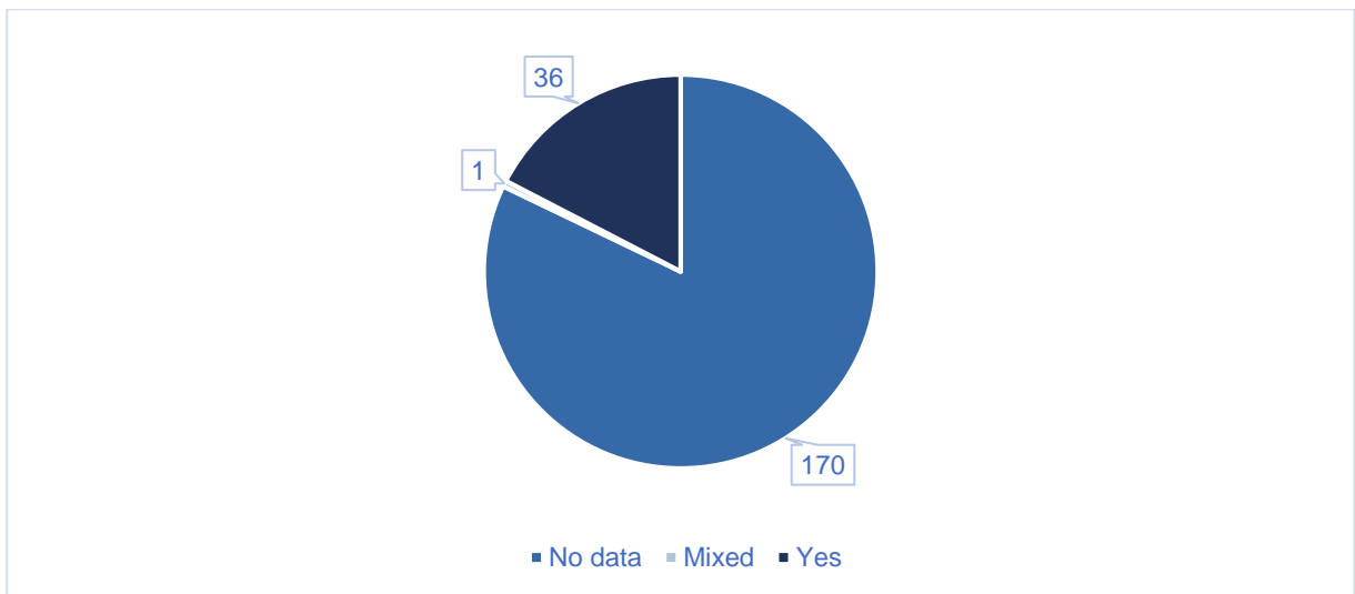
Figure 8 Machine readability
