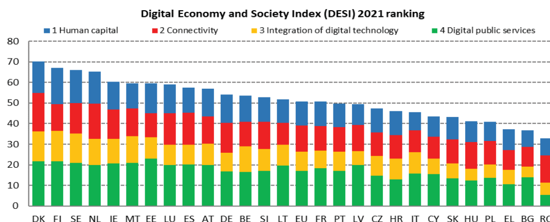
Chart 2: DESI 2021 ranking
