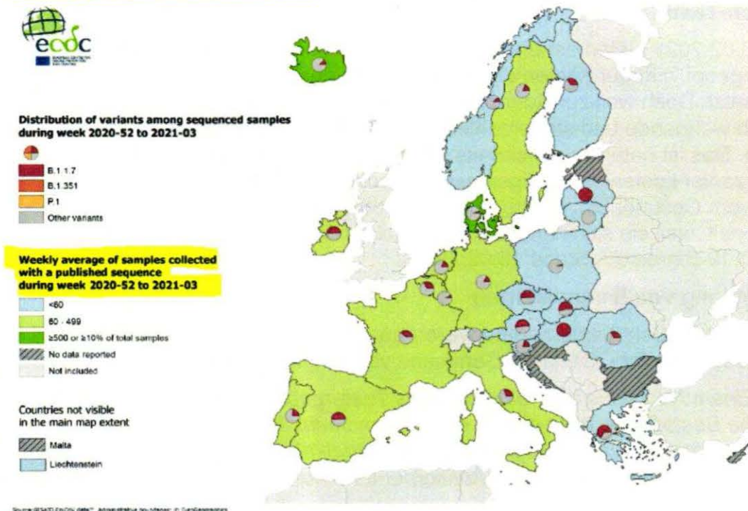
Figure 1. Distribution of SARS-CoV-2 variants and average number of samples sequenced in EU/EEA countries, weeks 2020-52 to 2021-03
