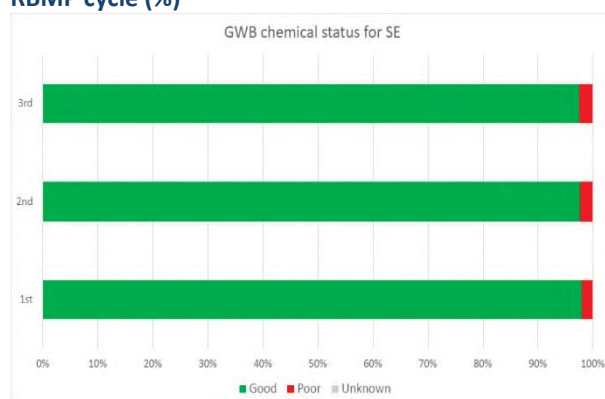
Figure 28: Chemical status of groundwater bodies in each RBMP cycle (%)
