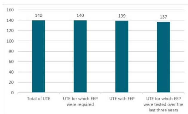
Figure 22: Situation regarding EEPs in Finland, 2022
