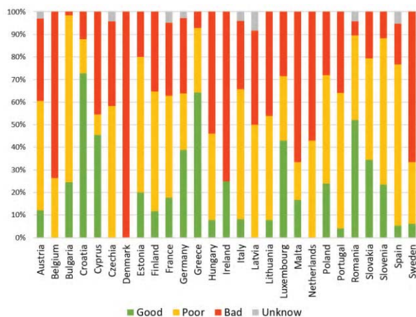
Figure 12: Conservation status of forests protected under the Habitats Directive per Member State (% of assessments), 2013–2018
