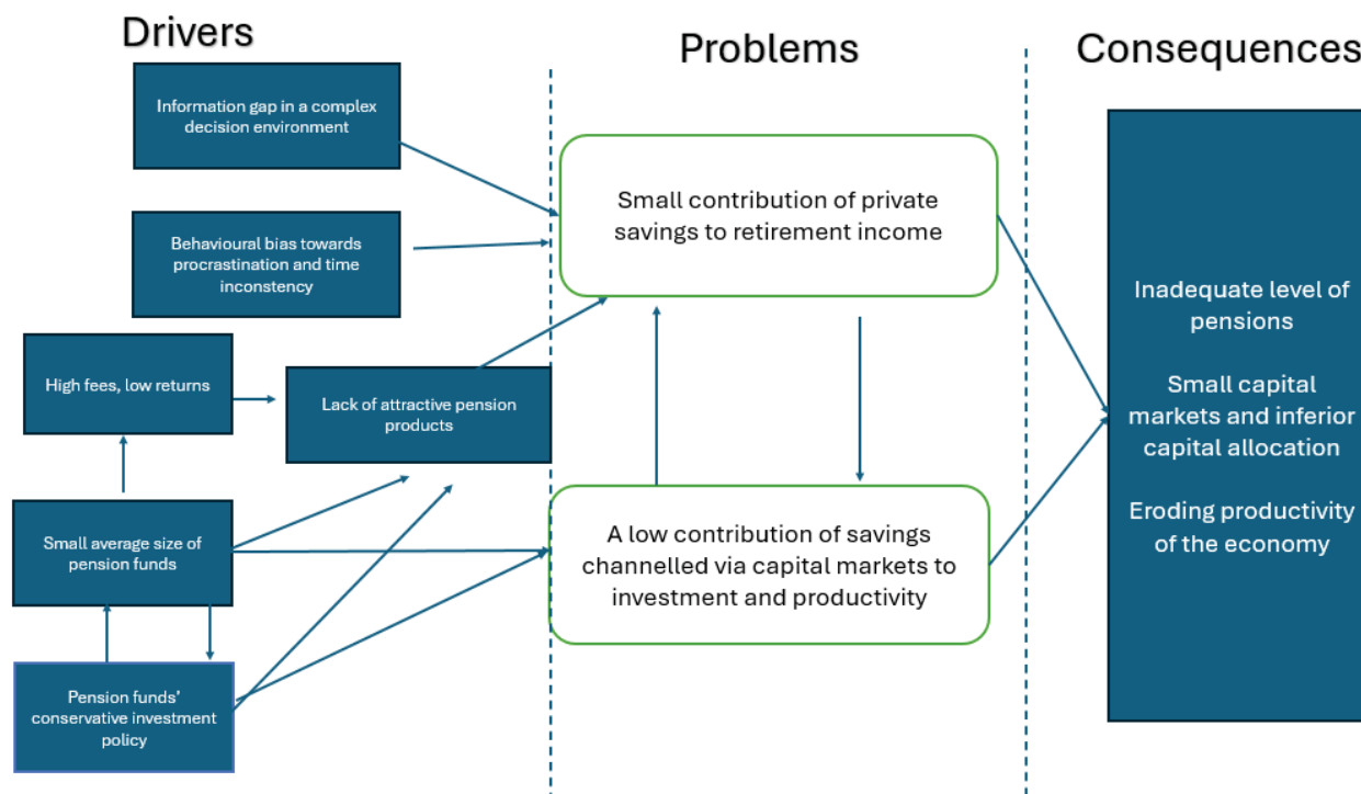
Figure 7: Problem tree
