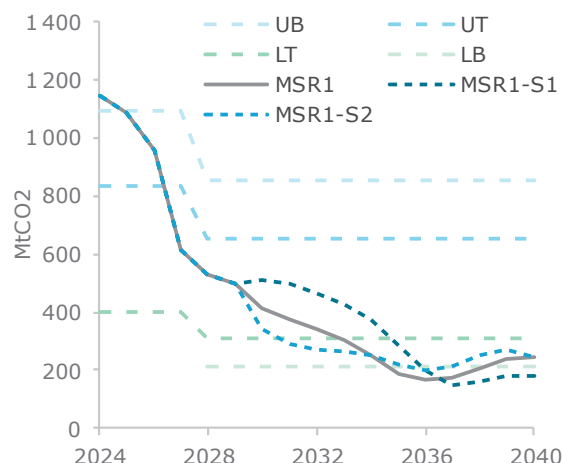
Figure 38: MSR sensitivity analysis - S1 & S2 - TNAC evolution for MSR1 (left) and MSR3 (right)
