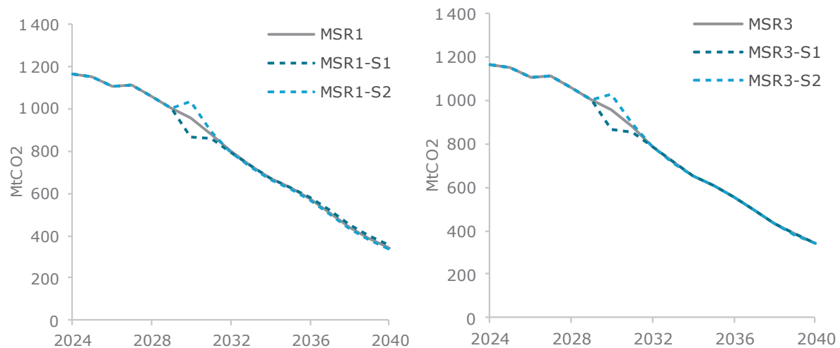
Figure 41: MSR sensitivity analysis - S1 & S2 – EU ETS emissions for MSR1 (left) and MSR3 (right)
