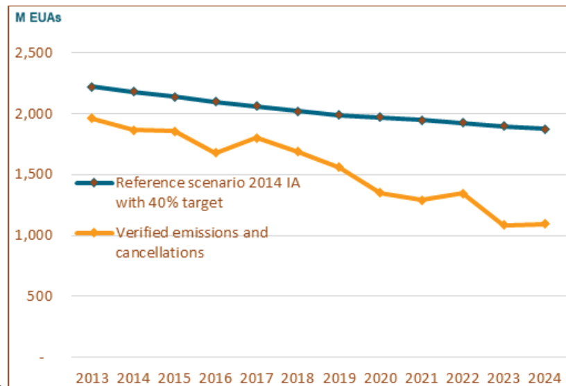
Figure 14: scenario from 2014 IA versus actual emissions
