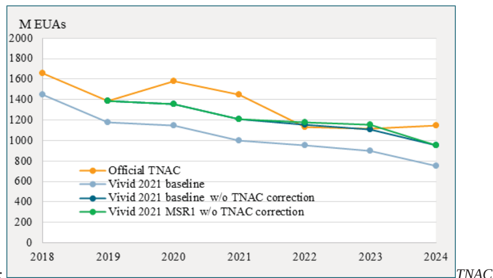
Figure 15: 2018 to 2024: Official data versus baseline and MSR1 from 2021 MSR Review
