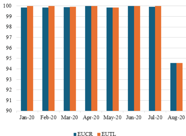
Figure 35: registry system from January to August 2020
