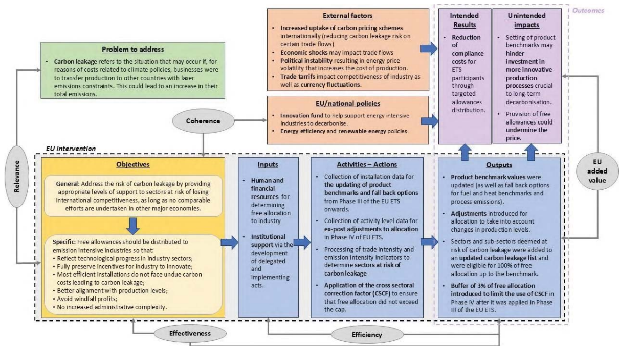
Figure 19: Intervention logic diagram (carbon leakage)
