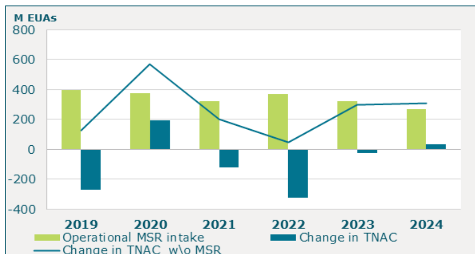
Figure 12: MSR intake; actual and ex-post baseline changes in TNAC
