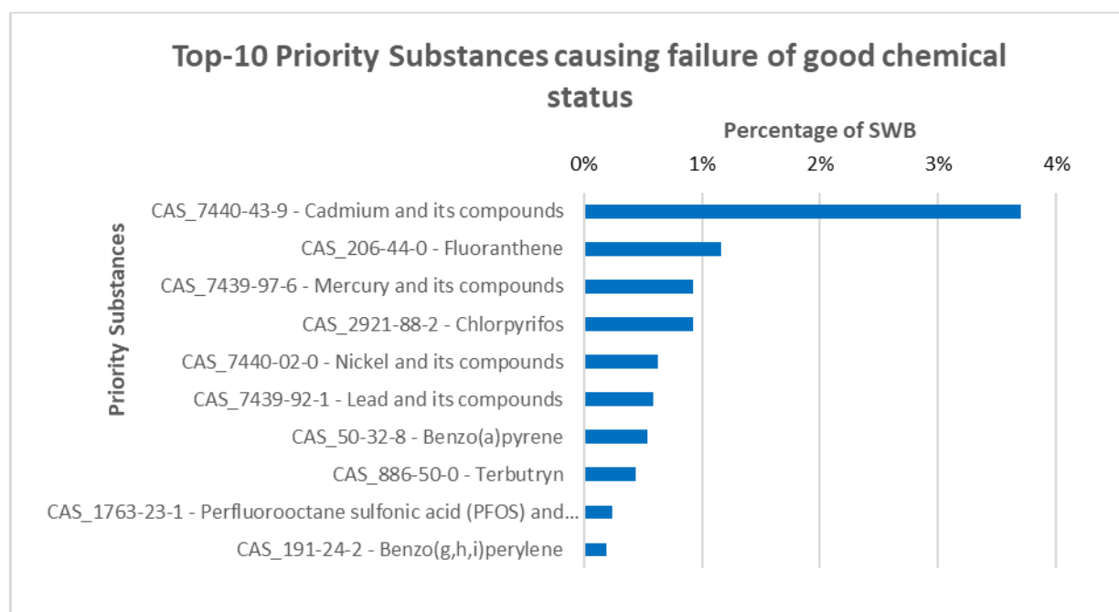
Figure 8. The top 10 priority substances causing failure to achieve good chemical status in surface water bodies in Portugal
