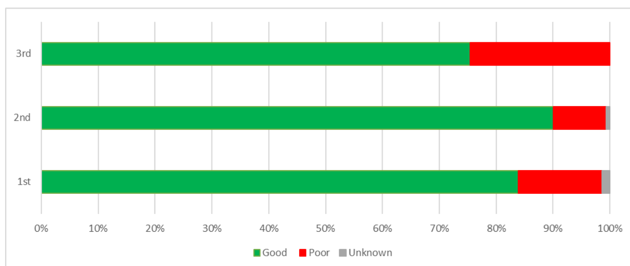
Figure 9. Chemical status of groundwater bodies in Portugal in the 1st, 2nd and 3rd RBMPs
