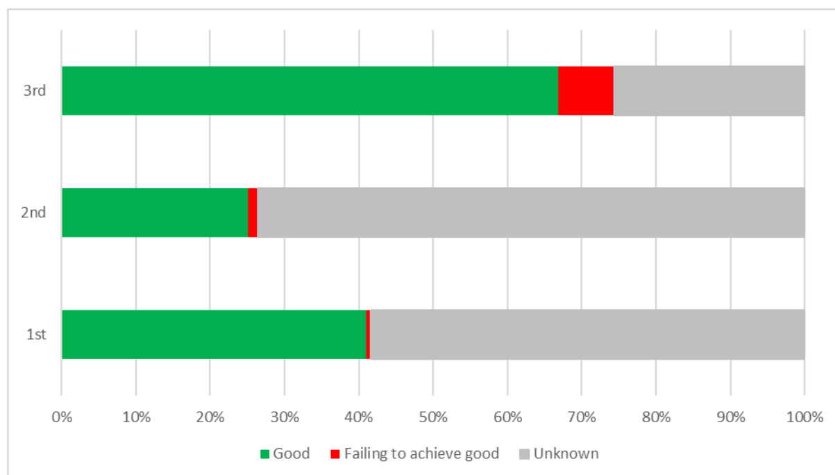
Figure 7. Chemical status of surface water bodies in Portugal in the 1st, 2nd and 3rd RBMPs
