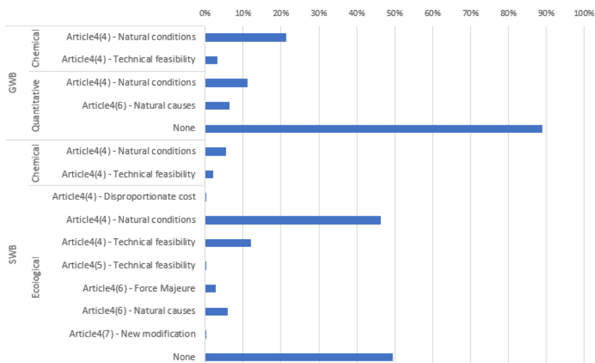
Figure 10. The use of exemptions under Article 4(4)-(7) WFD in surface water bodies (SWBs) and groundwater bodies (GWBs) in Portugal. The figure shows the proportion of water bodies for each type of exemption.
